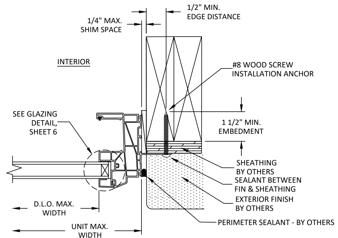
D 3 HORIZONTAL SECTION NAIL FIN INSTALLATION WOOD SUBSTRATE
