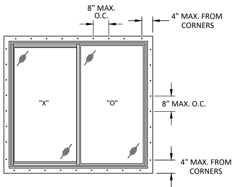
TYPICAL ANCHOR LAYOUT NAIL FIN INSTALLATION
