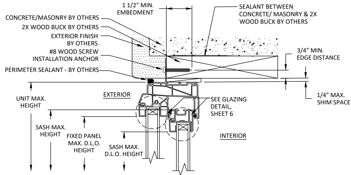
A 3 VERTICAL SECTION NAIL FIN INSTALLATION WOOD BUCK
