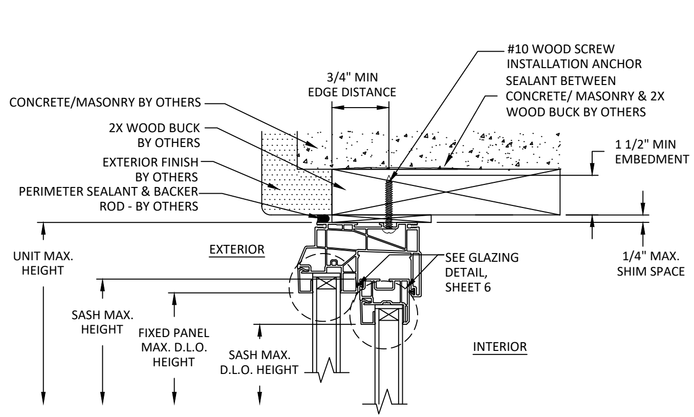
A 4 VERTICAL SECTION THROUGH FRAME INSTALLATION WOOD BUCK
