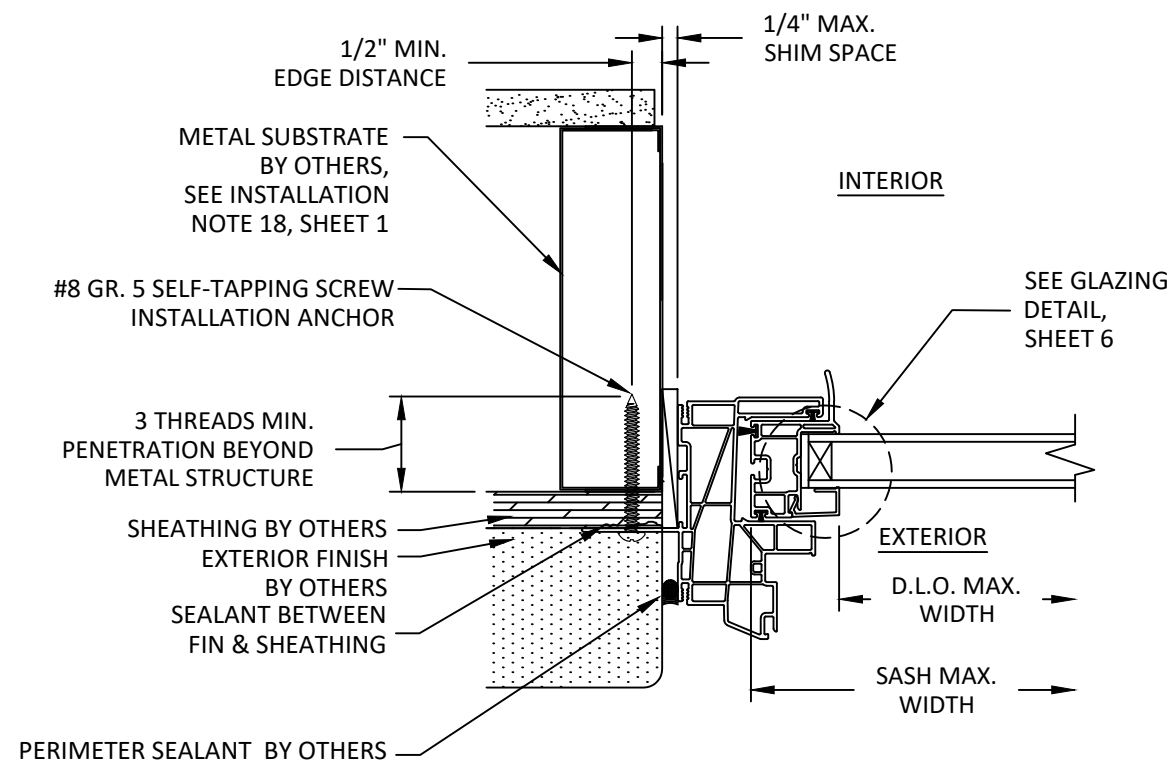
B 3 HORIZONTAL SECTION NAIL FIN INSTALLATION METAL SUBSTRATE
