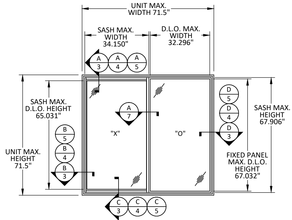
TYPICAL ELEVATION HORIZONTAL SLIDER
