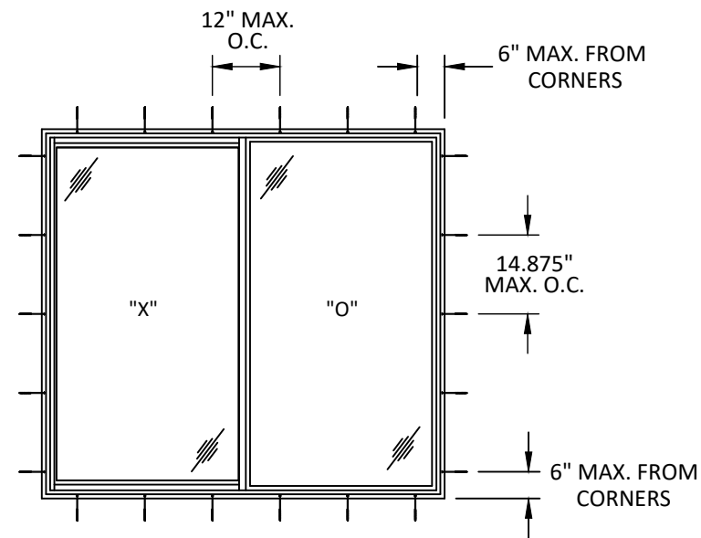
TYPICAL ANCHOR LAYOUT THROUGH FRAME AND CLIP INSTALLATION
